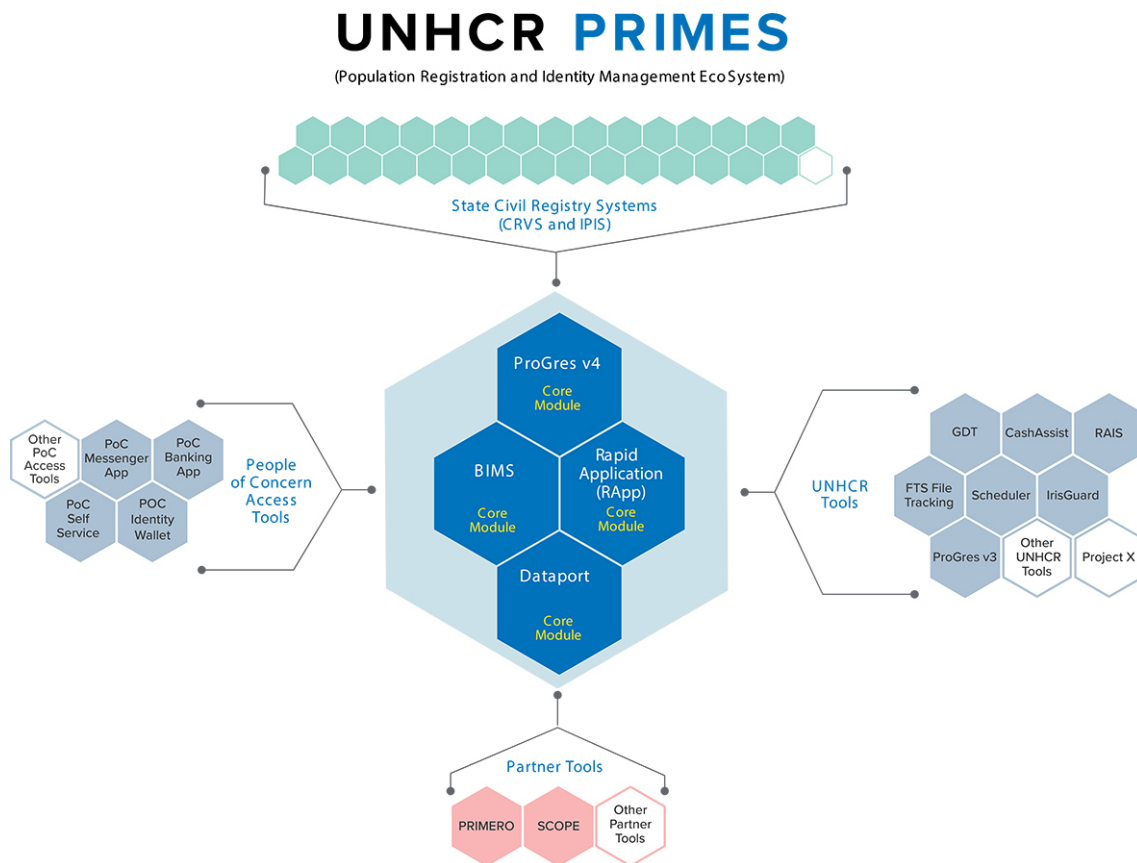
Figure 2: The PRIMES ecosystem of tools (Source UNHCR https://www.unhcr.org/primes.html ).
